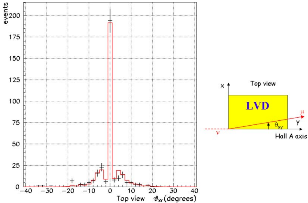
Fig. 11. Distribution of the “top” projection of the angle between the reconstructed muon track and the main axis of the LNGS hall: comparison between the data (black crosses) and MC simulation (red line). In the right picture there is a description of the considered angle \theta_{xy}
