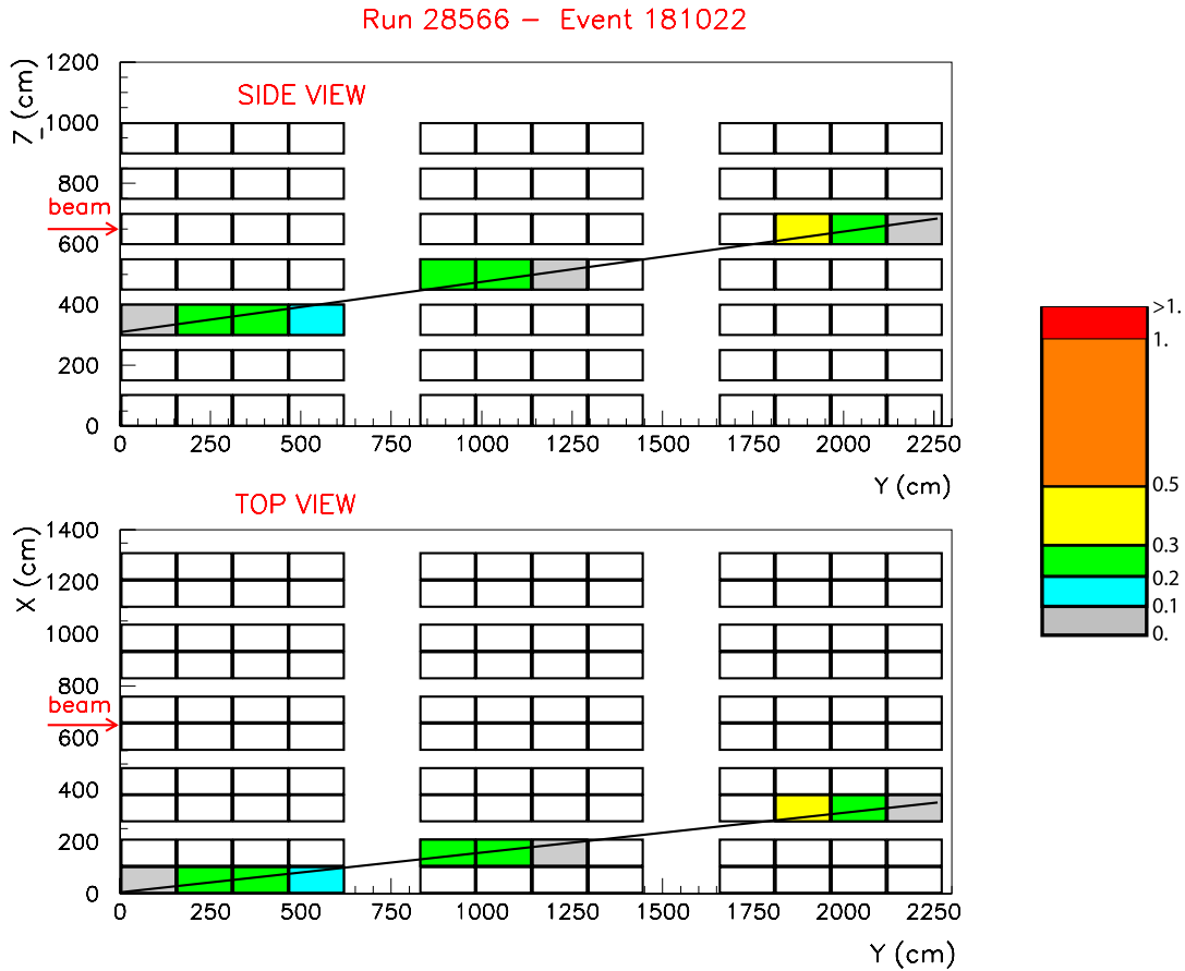
Fig. 6. Display of a CNGS events: typical charged current interaction in the rock upstream LVD, producing a muon that goes through the detector. The colours represent the amount of energy released in the scintillation counters, summed along each projected view; the legend is expressed in GeV. The black straight line is the result of a linear fit to the hit counters
