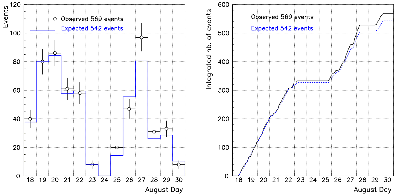
Fig. 5. Comparison between the expected and detected number of events during Run1. In the left panel there is the number of events per day: observed ( black circles ) and expected ( blue line ). In the right one the integrated number of events: observed ( black solid line ) and expected ( blue dashed line )
