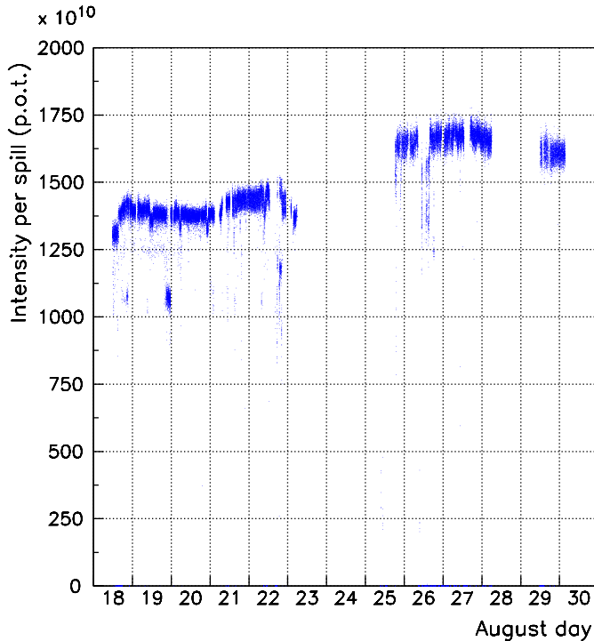
Fig. 1. Beam intensity (in protons on target) per each spill of Run1
