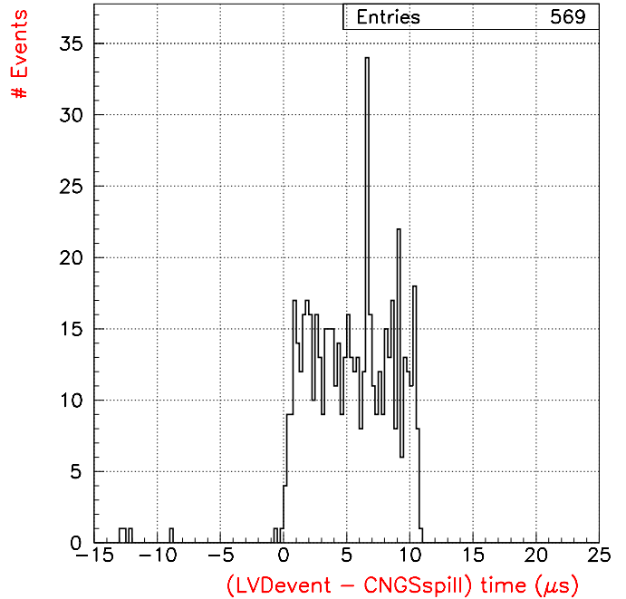
Fig. 4. Distribution of the detection time of the 569 CNGS events, with respect to the initial time of the beam spill
