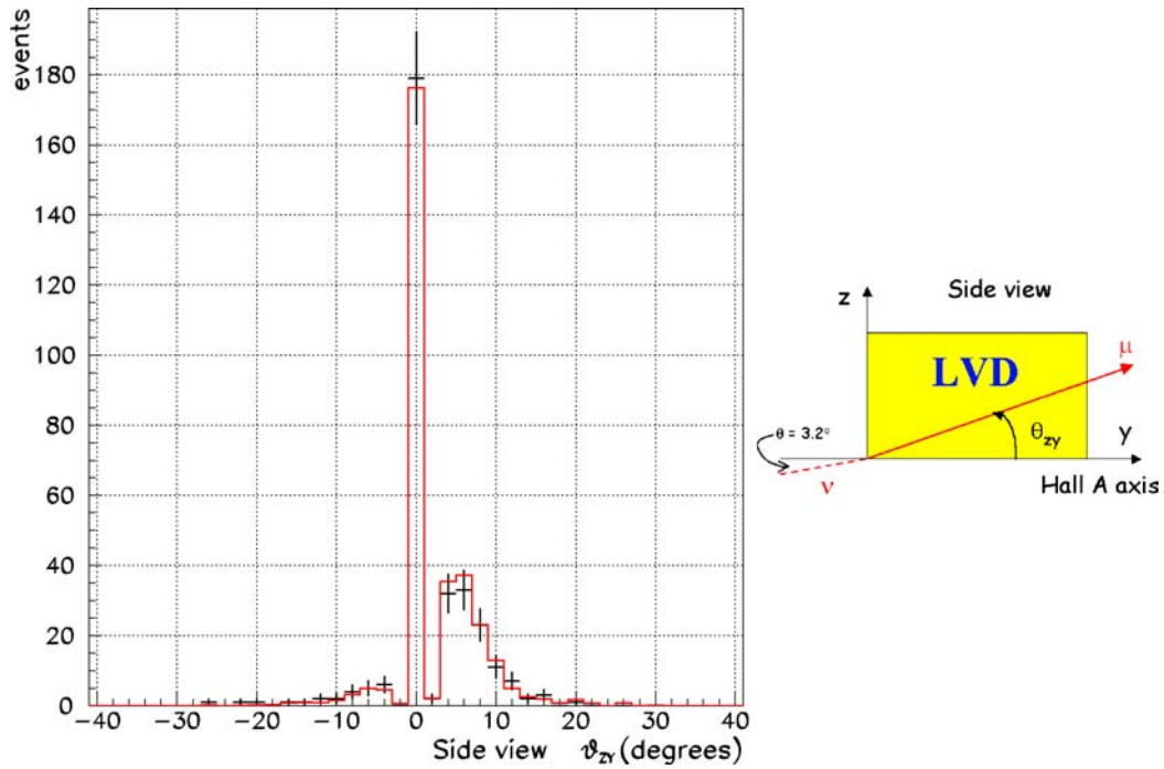
Fig. 10. Distribution of the “side” projection of the angle between the reconstructed muon track and the main axis of the LNGS hall: comparison between the data (black crosses) and MC simulation (red line). In the right picture there is a description of the considered angle \theta_{zy}
