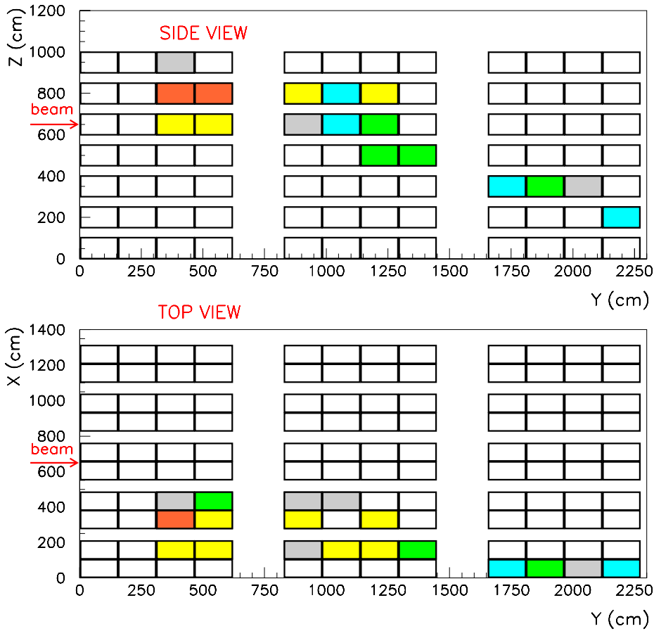
Fig. 7. Display of a CNGS events: neutrino interaction inside the LVD detector. The colours represent the amount of energy released in the scintillation counters, summed along each projected view; the legenda is the same as in Fig. 6
